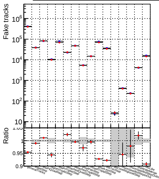
Number —●— DQM_CKF_TT_retrainOldFiles125_v2_prelimWPM_epoch0
