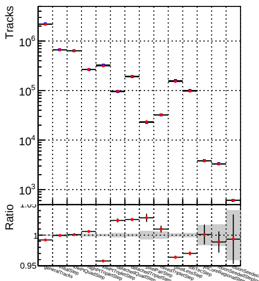
Number of fake tracks vs collection Legend: DQM_CKF_TTbase (blue line with dots), DQM_CKF_TT_retrainOldFiles125_v2_prelimWPM_epoch0 (red line with dots)
