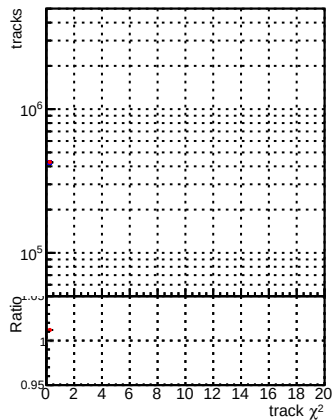
N of reco track vs. \chi^2 for DQM CKF TTbase and DQM CKF TT_retrainOldFiles125_v2_prelimWPM_epoch0
