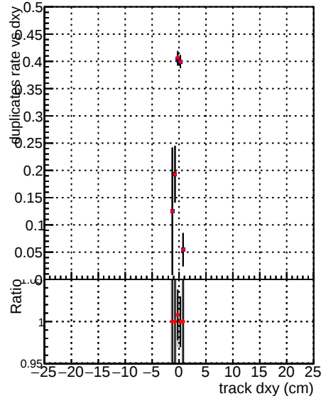
—●— DQM_CKF_TTbase —●— DQM_CKF_TT_retrainOldFiles125_v2_prelimWPM_epoch0
