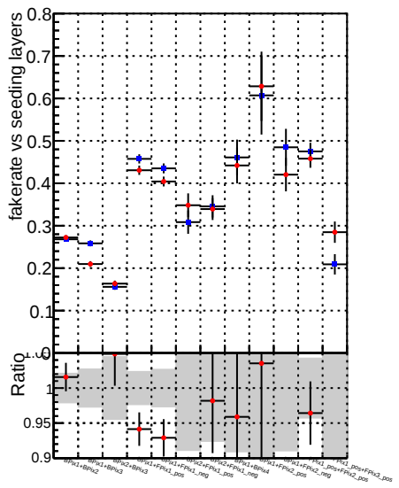
Fake rate vs. seed rate vs seeding layers
