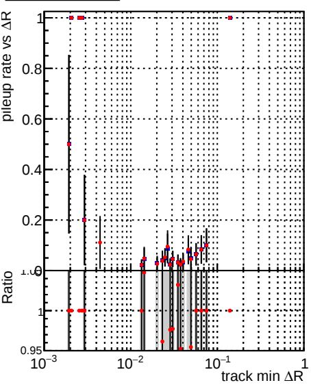
Legend: DQM_CKF_TTbase (blue stars), DQM_CKF_TT_retrainOldFiles125_v2_prelimWPM_epoch0 (red stars)
