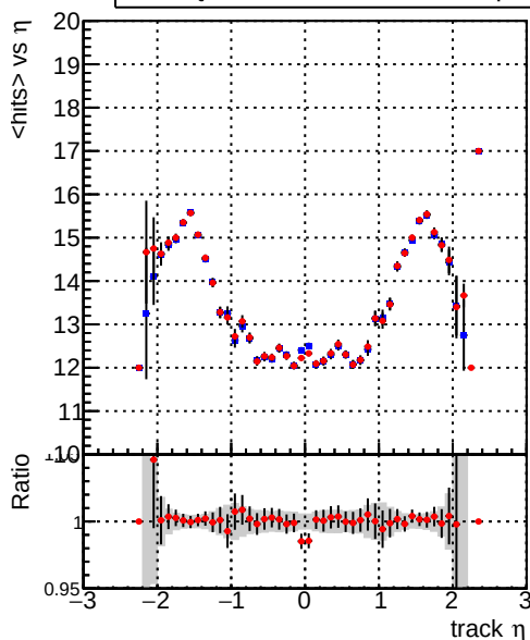
mean hits vs \eta Legend: DQM_CKF_TTbase (blue line with dots), DQM_CKF_TT_retrainOldFiles125_v2_prelimWPM_epoch0 (red line with dots)
