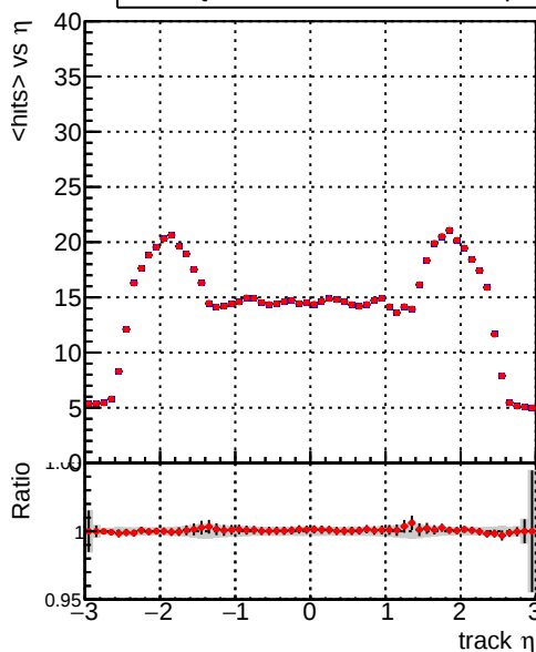
mean hits — DQM_CKF_TTbase — DQM_CKF_TT_retrainOldFiles125_v2_prelimWPM_epoch0
