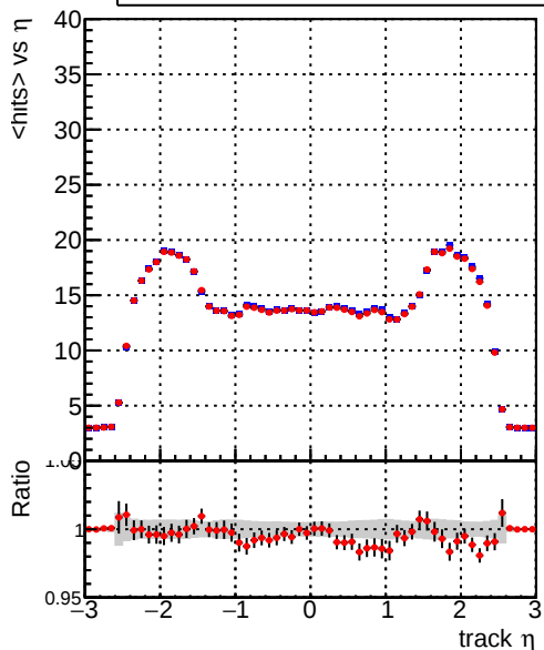
mean hits — DQM_CKF_TTbase — DQM_CKF_TT_retrainOldFiles125_v2_prelimWPM_epoch0
