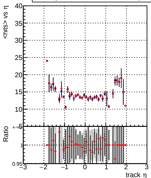
mean hits vs \eta Legend: DQM_CKF_TTbase (blue line with markers), DQM_CKF_TT_retrainOldFiles125_v2_prelimWPM_epoch0 (red line with markers)
