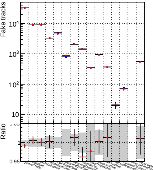
Number Model 1 DQM_CKF_TT_retrainOldFiles125_v2_prelimWPM_epoch0
