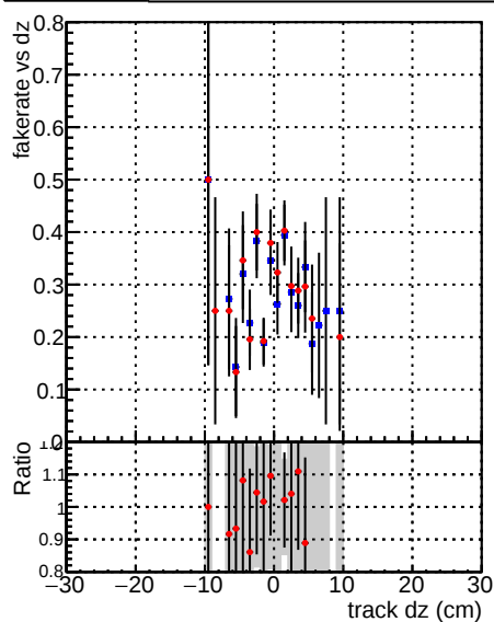
—●— DQM_CKF_TTbase —●— DQM_CKF_TT_retrainOldFiles125_v2_prelimWPM_epoch0
