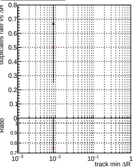
Legend: DQM_CKF_TTbase (blue circles), DQM_CKF_TT_retrainOldFiles125_v2_prelimWPM_epoch0 (red circles)
