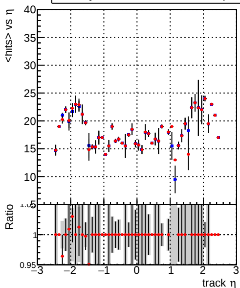
mean hit Legend: DQM_CKF_TTbase (blue line with markers), DQM_CKF_TT_retrainOldFiles125_v2_prelimWPM_epoch0 (red line with markers)
