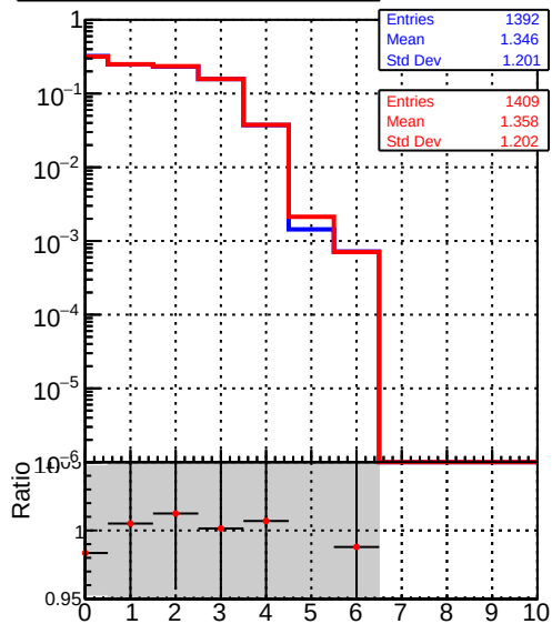
mean hit — DQM_CKF_TTbase — DQM_CKF_TT_retrainOldFiles125_v2_prelimWPM_epoch0
