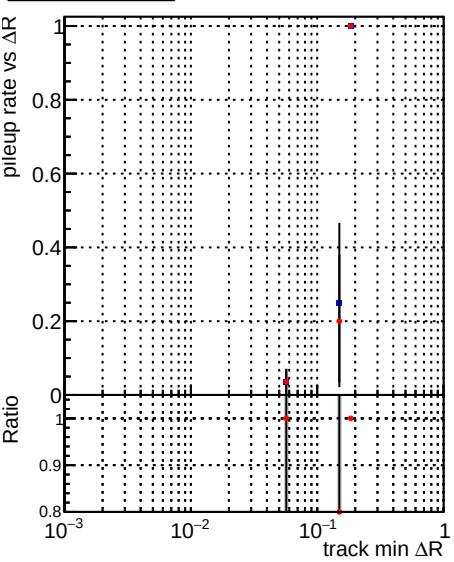
Legend: DQM_CKF_TTbase (blue), DQM_CKF_TT_retrainOldFiles125_v2_prelimWPM_epoch0 (red)
