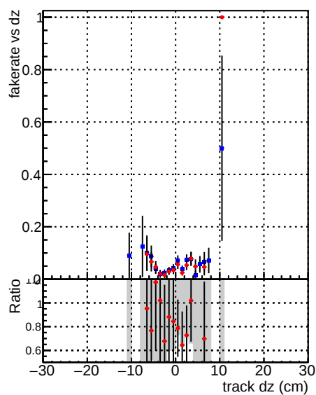
Fake rate vs dz —●— DQM_CKF_TTbase —●— DQM_CKF_TT_retrainOldFiles125_v2_prelimWPM_epoch0
