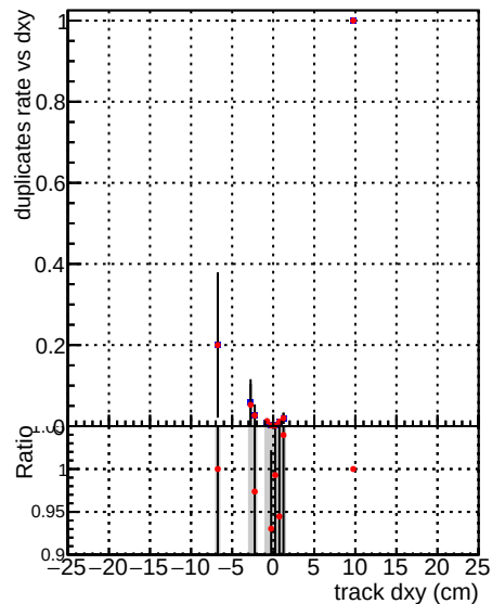
—●— DQM_CKF_TTbase —●— DQM_CKF_TT_retrainOldFiles125_v2_prelimWPM_epoch0
