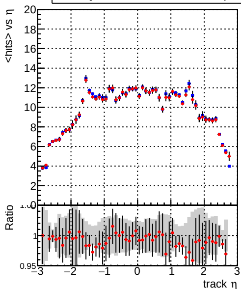
mean hits vs \eta Legend: DQM_CKF_TTbase (blue line), DQM_CKF_TT_retrainOldFiles125_v2_prelimWPM_epoch0 (red line)
