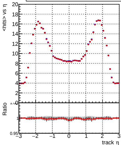
mean hits vs \eta — DQM_CKF_TTbase — DQM_CKF_TT_retrainOldFiles125_v2_prelimWPM_epoch0
