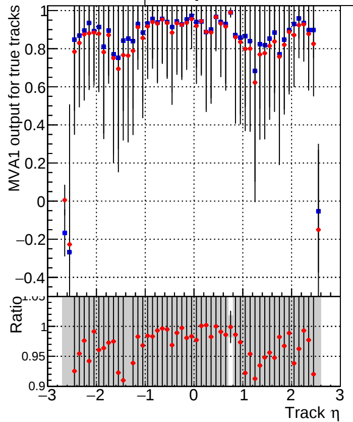
MVA1 of associated tracks (recoToSim) vs. track \eta Legend: ■ DQM_CKF_TTbase ◆ DQM_CKF_TT_retrainOldFiles125_v2_prelimWPM_epoch0
