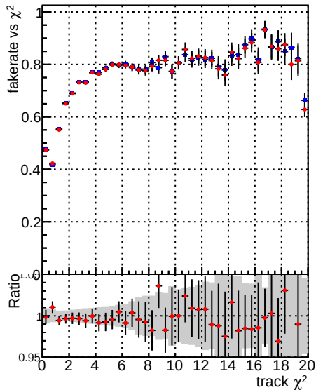
Fake rate vs. \chi^2 Legend: DQM CKF TTbase (blue diamonds) DQM CKF TT_retrainOldFiles125_v2_prelimWPM_epoch0 (red circles)
