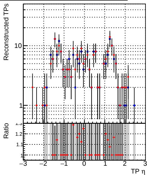
N of simulated tracks vs TP \eta Legend: —•— DQM_CKF_TTbase —•— DQM_CKF_TT_retrainOldFiles125_v2_prelimWPM_epoch0
