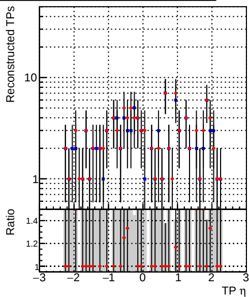
—•— DQM_CKF_TTbase —•— DQM_CKF_TT_retrainOldFiles125_v2_prelimWPM_epoch0
