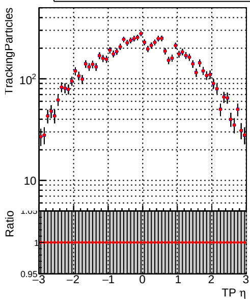
N of simulated tracks vs \eta Legend: DQM_CKF_TTbase (blue line), DQM_CKF_TT_retrainOldFiles125_v2_prelimWPM_epoch0 (red line)
