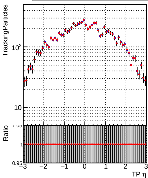
N of simulated tracks vs \eta Legend: DQM_CKF_TTbase (blue squares), DQM_CKF_TT_retrainOldFiles125_v2_prelimWPM_epoch0 (red diamonds)
