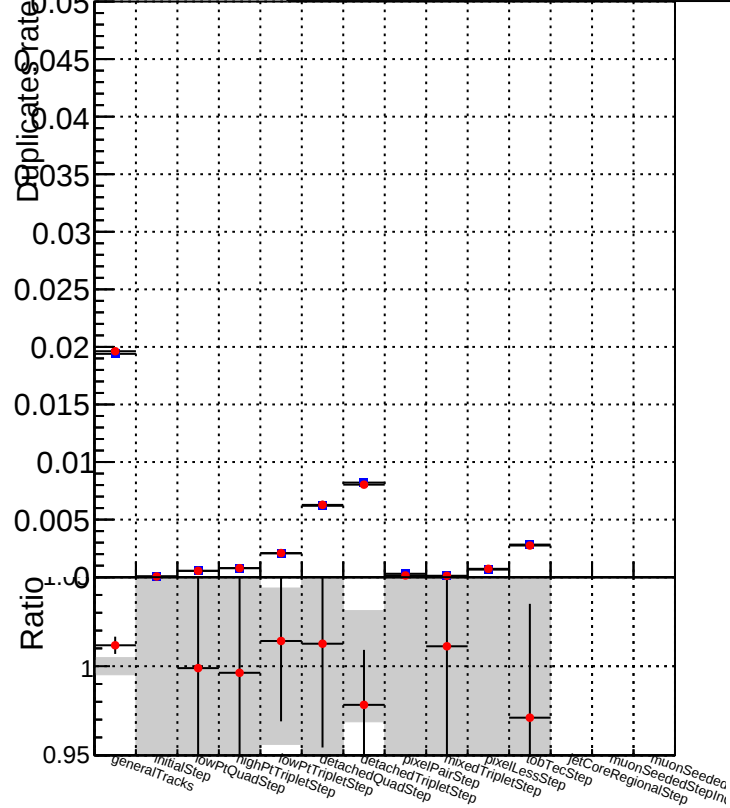
Duplicates rate vs collection Legend: DQM_CKF_TTbase (Blue square) DQM_CKF_TT_retrainOldFiles125_v2_prelimWPM_epoch0 (Red circle)
