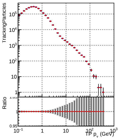
—•— DQM_CKF_TTbase —•— DQM_CKF_TT_retrainOldFiles125_v2_prelimWPM_epoch0
