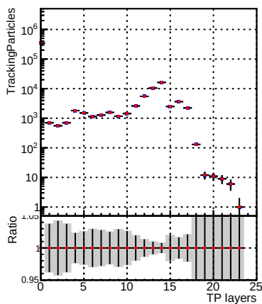
N of sim DQM_CKF_TTbase DQM_CKF_TT_retrainOldFiles125_v2_prelimWPM_epoch0
