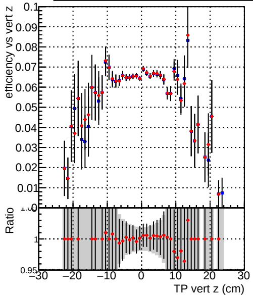
Efficiency vs. TP vert z (cm) — DQM_CKF_TTbase — DQM_CKF_TT_retrainOldFiles125_v2_prelimWPM_epoch0
