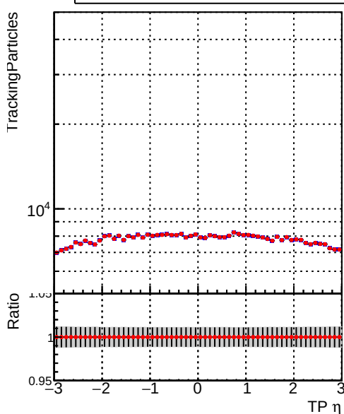
N of simulated tracks vs TP \eta — DQM_CKF_TTbase — DQM_CKF_TT_retrainOldFiles125_v2_prelimWPM_epoch0
