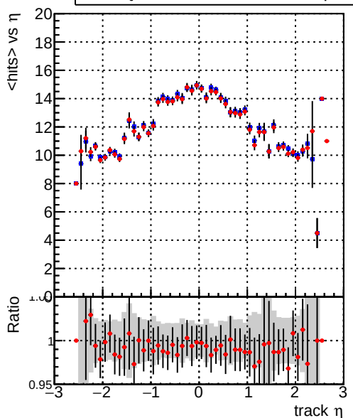
mean hits vs \eta Legend: DQM_CKF_TTbase (blue line), DQM_CKF_TT_retrainOldFiles125_v2_prelimWPM_epoch0 (red line)
