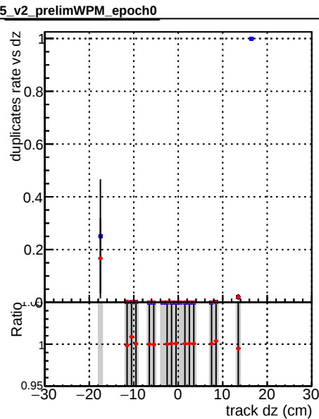
—●— DQM_CKF_TTbase —●— DQM_CKF_TT_retrainOldFiles125_v2_prelimWPM_epoch0
