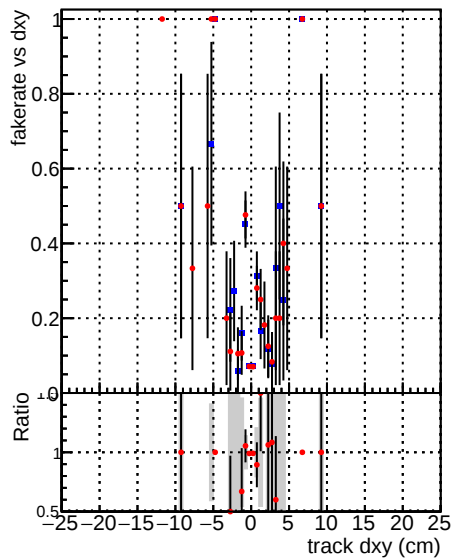
—●— DQM_CKF_TTbase —●— DQM_CKF_TT_retrainOldFiles125_v2_prelimWPM_epoch0
