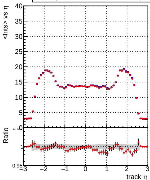
— DQM_CKF_TTbase — DQM_CKF_TT_retrainOldFiles125_v2_prelimWPM_epoch0 mean hits > \eta
