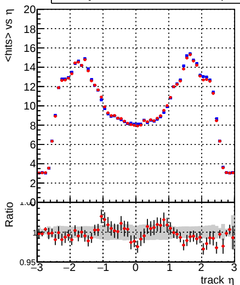
— DQM_CKF_TTbase — DQM_CKF_TT_retrainOldFiles125_v2_prelimWPM_epoch0 mean hits > \eta
