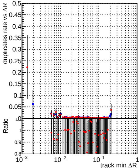
Legend: —•— DQM_CKF_TTbase —•— DQM_CKF_TT_retrainOldFiles125_v2_prelimWPM_epoch0
