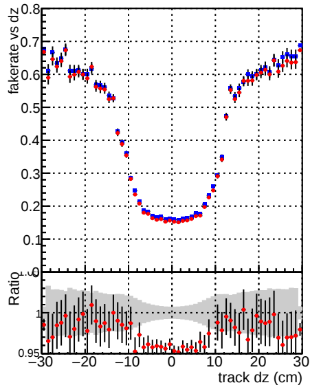
—●— DQM CKF QCDHighPt_base —●— DQM CKF QCDHighPt_retrainOldFiles125_v2_prelimWPM_epoch4
