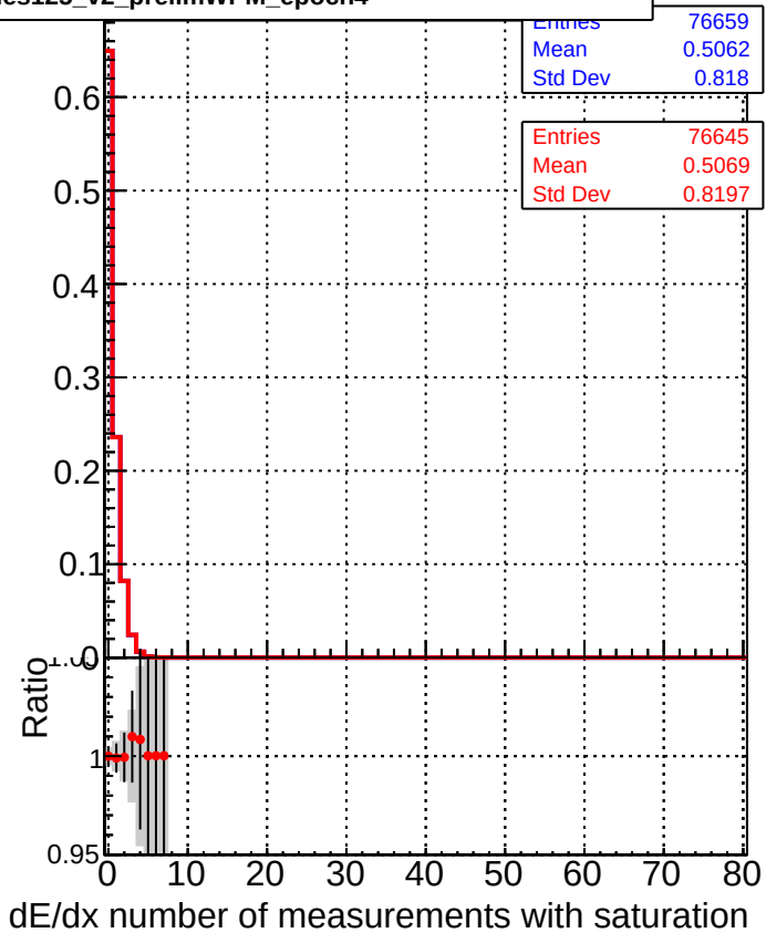
DQM_CKF_QCDHighPt_base DQM_CKF_QCDHighPt_retrainOldFiles125_v2_prelimWPM_epoch4
