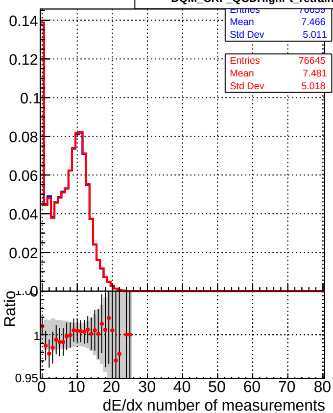
DQM_CKF_QCDHighPt_base DQM_CKF_QCDHighPt_retrainOldFiles125_v2_prelimWPM_epoch4
