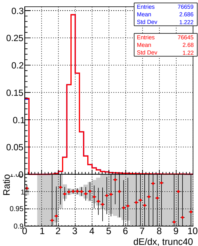
DQM_CKF_QCDHighPt_base DQM_CKF_QCDHighPt_retrainOldFiles125_v2_prelimWPM_epoch4
