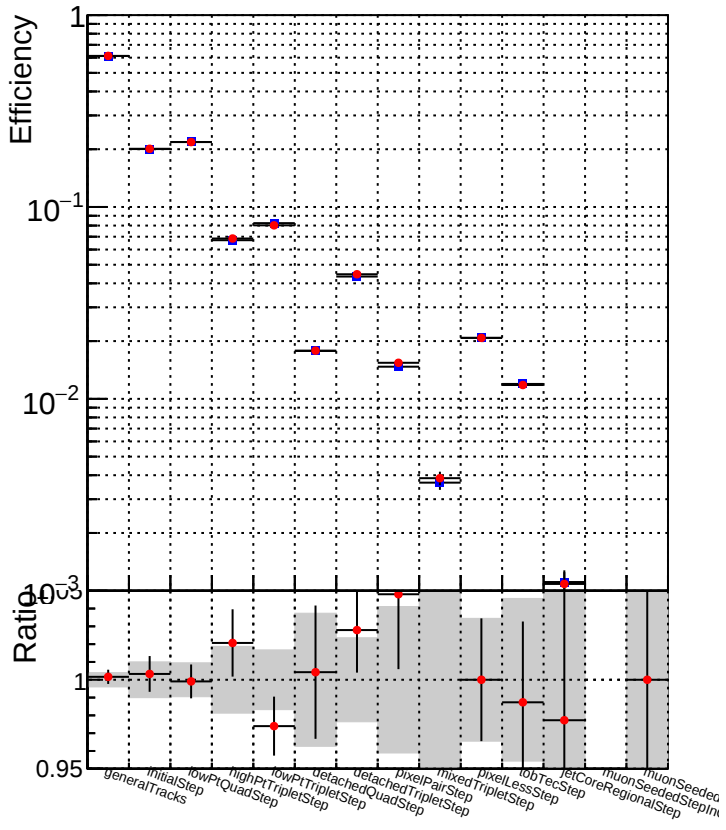
DQM_CKF_QCDHighPt_base DQM_CKF_QCDHighPt_retrainOldFiles125_v2_prelimWPM_epoch3
