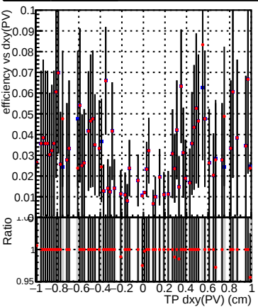
Efficiency vs Dxy(PV) Legend: DQM_CKF_QCDHighPt_base (blue squares), DQM_CKF_QCDHighPt_retrainOldFiles125_v2_prelimWPM_epoch3 (red circles)
