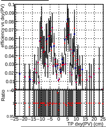
Efficiency vs Dxy(PV) Legend: DQM_CKF_QCDHighPt_base (blue squares), DQM_CKF_QCDHighPt_retrainOldFiles125_v2_prelimWPM_epoch3 (red circles)
