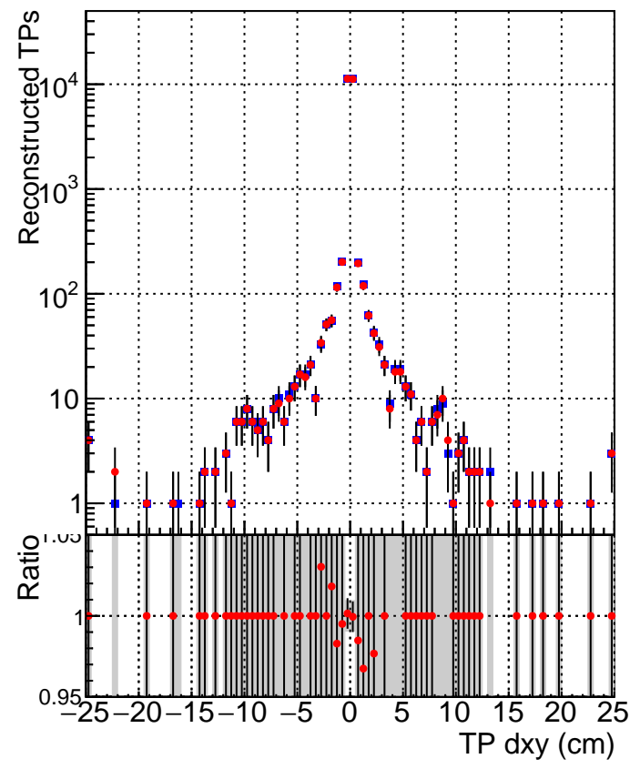
—■— DQM_CKF_QCDHighPt_base —●— DQM_CKF_QCDHighPt_retrainOldFiles125_v2_prelimWPM_epoch3
