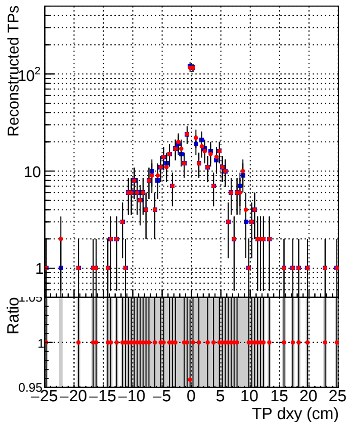
■ DQM_CKF_QCDHighPt_base ■ DQM_CKF_QCDHighPt_retrainOldFiles125_v2_prelimWPM_epoch3
