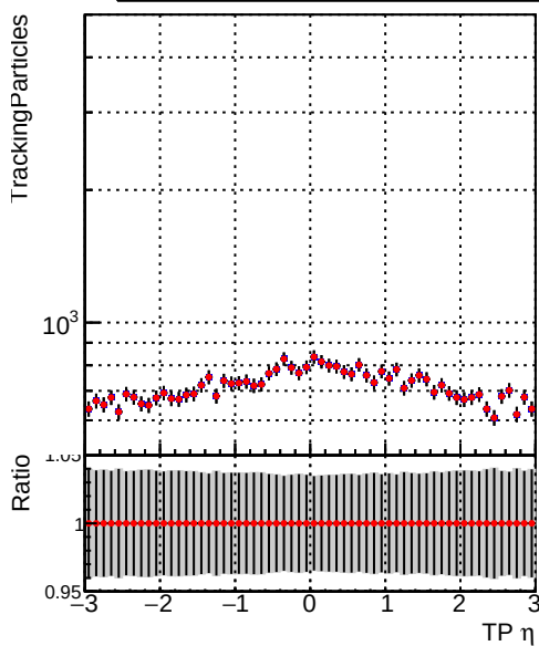
Legend: DQM_CKF_QCDHighPt_base (blue line), DQM_CKF_QCDHighPt_retrainOldFiles125_v2_prelimWPM_epoch3 (red line)
