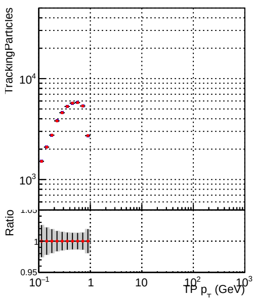
Legend: DQM_CKF_QCDHighPt_base (blue line), DQM_CKF_QCDHighPt_retrainOldFiles125_v2_prelimWPM_epoch3 (red line)
