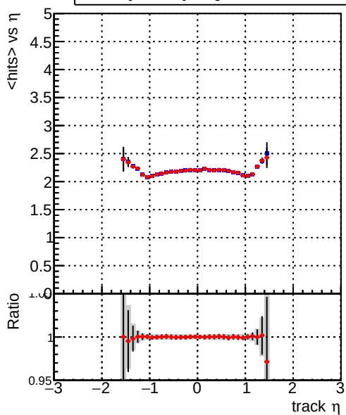
mean hits vs \eta Legend: DQM_CKF_QCDHighPt_base (blue line with points), DQM_CKF_QCDHighPt_retrainOldFiles125_v2_prelimWPM_epoch3 (red line with points)
