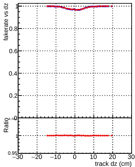
Fake rate vs dz —●— DQM CKF QCDHighPt_base —●— DQM CKF QCDHighPt_retrainOldFiles125_v2_prelimWPM_epoch3
