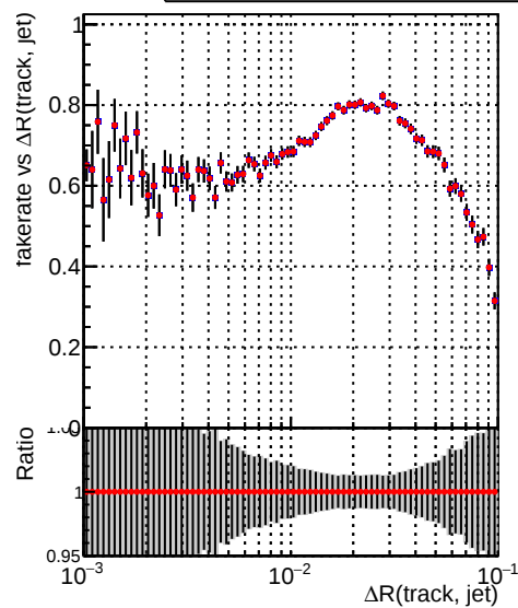
DQM_CKF_QCDHighPt_base
