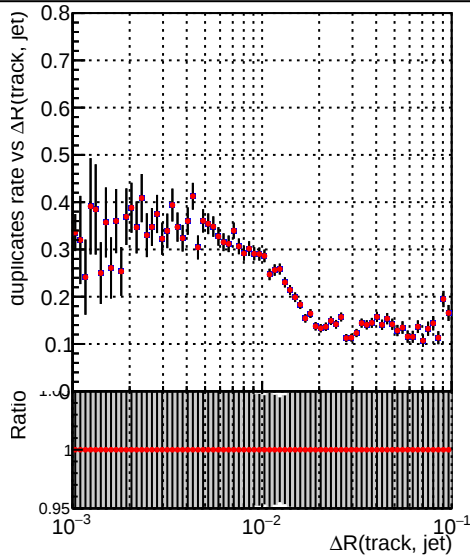
DQM_CKF_QCDHighPt_retrainOldFiles125_v2_prelimWPM_epoch3
