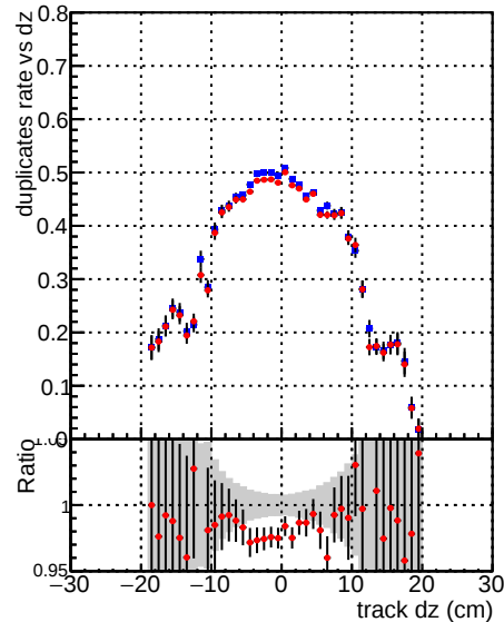
—●— DQM_CKF_QCDHighPt_base —●— DQM_CKF_QCDHighPt_retrainOldFiles125_v2_prelimWPM_epoch3
