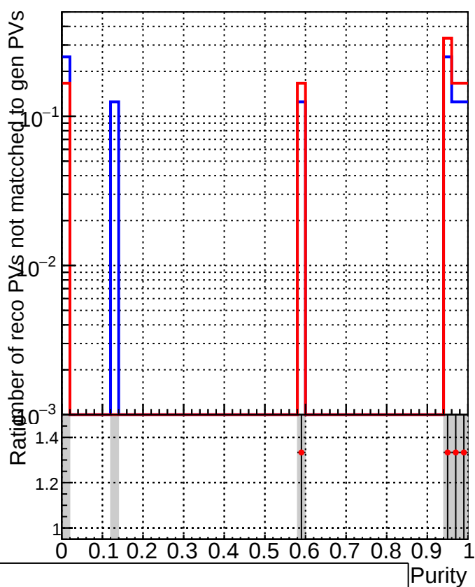
RecoPVAssoc2GenPVNotMatched_Purity
