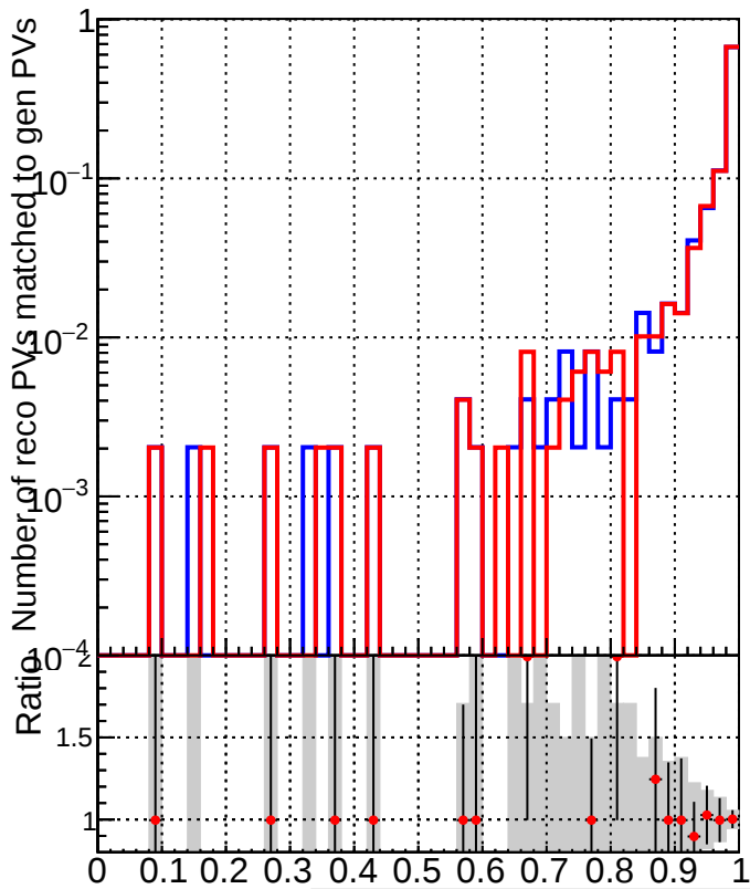
RecoPVAssoc2GenPVMatched_Purity
