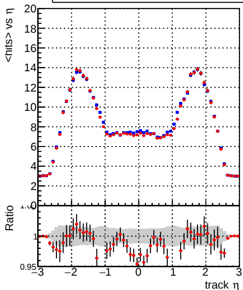
mean hits vs \eta — DQM_CKF_QCDHighPt_base — DQM_CKF_QCDHighPt_retrainOldFiles125_v2_prelimWPM_epoch3
