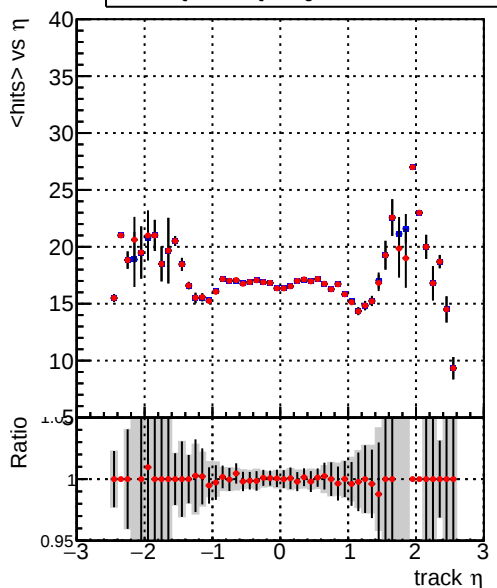
mean hits vs \eta — DQM_CKF_QCDHighPt_base — DQM_CKF_QCDHighPt_retrainOldFiles125_v2_prelimWPM_epoch3
